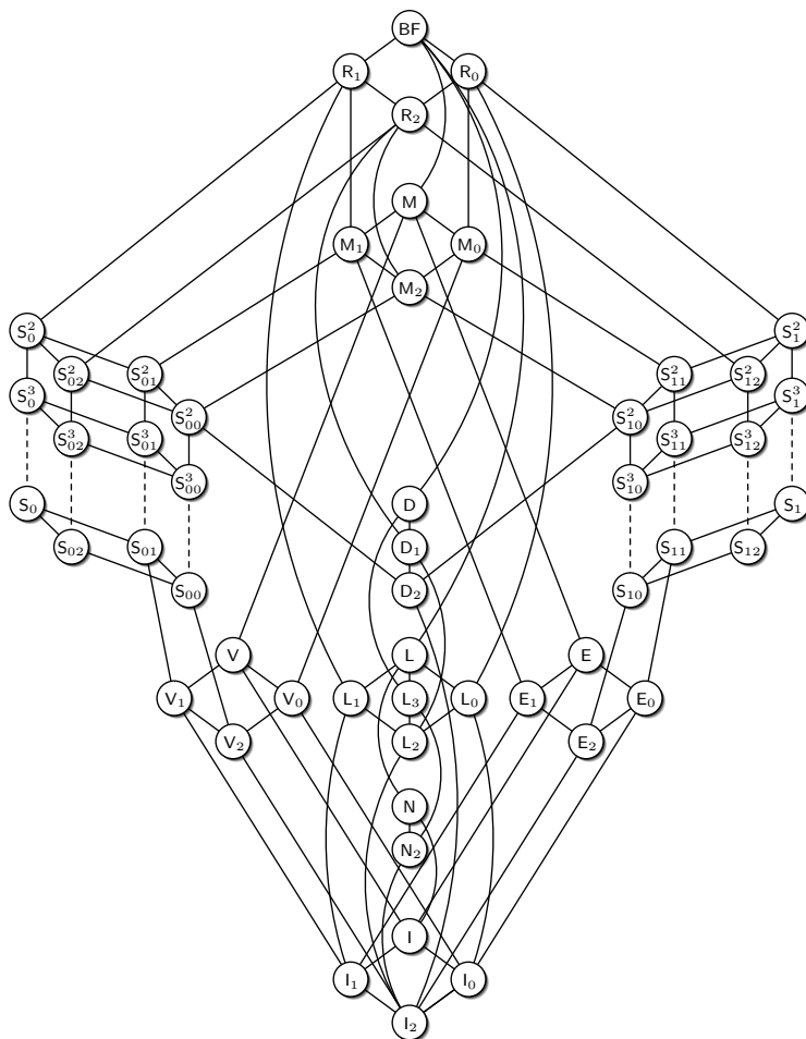
Figure 1: Post's lattice
