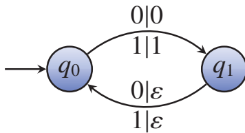
Figure 9: FST for \text{zip}(u, v) \triangleright u .
