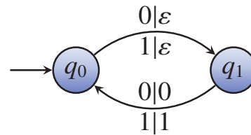
Figure 10: FST for \text{zip}(u, v) \triangleright v .
