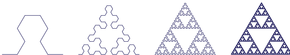
Figure 5: Initial approximations of the Sierpiński arrowhead curve [47].
