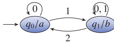
Figure 14: An example of a mix-DFAO.
