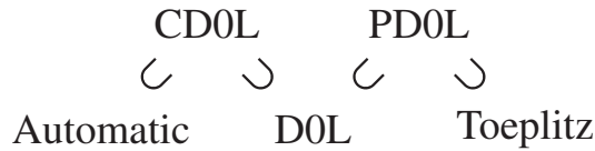
Figure 1: Some inclusions between stream families.
