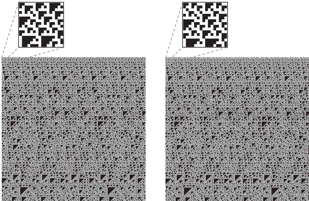
Figure 17: Comparing the ‘fingerprints’ \Delta^\omega(\mathbf{S}) and \Delta^\omega(\mathbf{W}) of the Sierpiński sequence \mathbf{S} (left), and the Mephisto Waltz \mathbf{W} . We find that \Delta^2(\mathbf{S}) = \Delta^3(\mathbf{W})!
