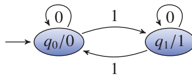
Figure 2: DFAO generating the Thue-Morse sequence.
